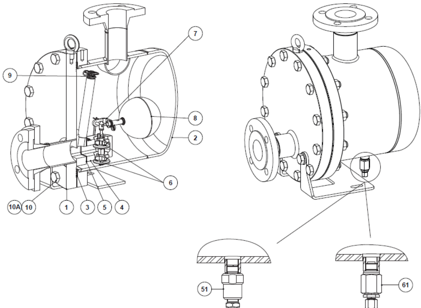
Optional blowdown valve (BDV); Manual
