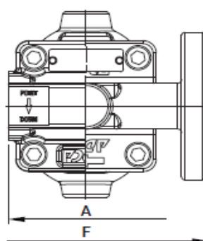
Inline design
