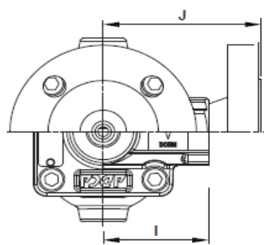
Angled design
