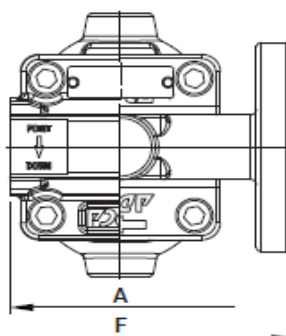
Inline design
