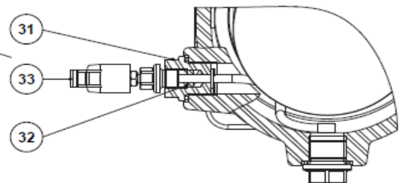
Optional float lifting lever (FLL)
