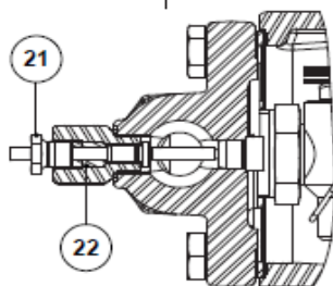
Optional steam lock release (SLR)
