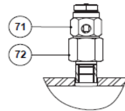
Optional vacuum breaker (VB21M)
