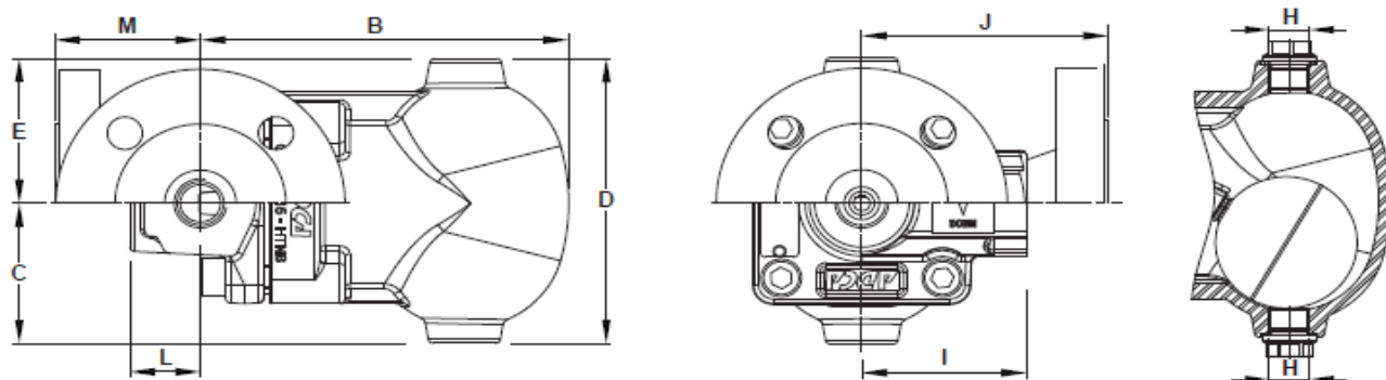
Angled design
