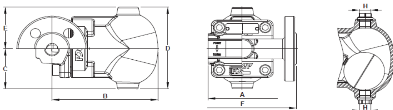
Inline design
