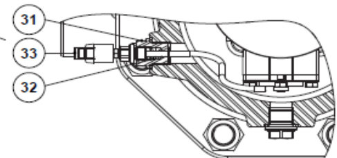
Optional float lifting lever (FLL)
