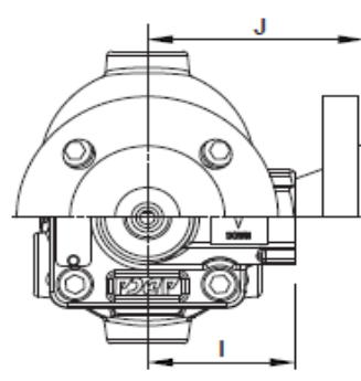
Angled design
