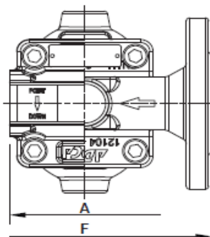
Inline design
