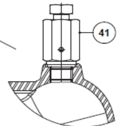
Optional hand vent valve (HVV)
