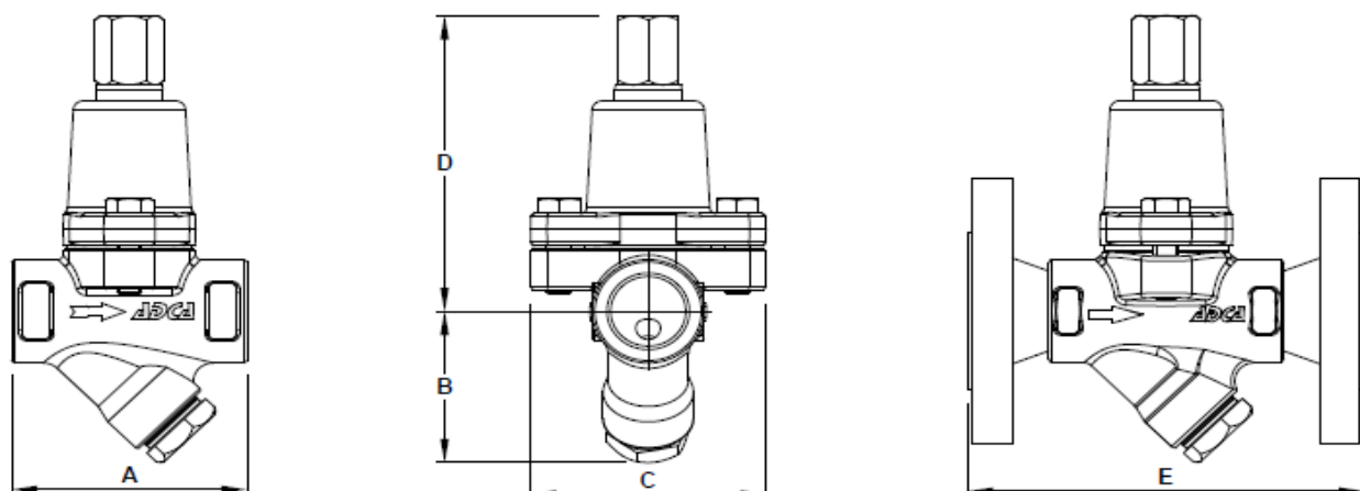
DIMENSIONS (mm)
