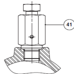
Optional hand vent valve (HVV)
