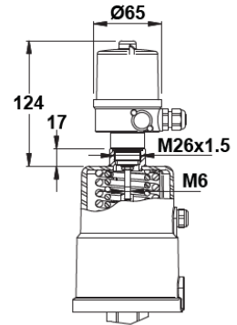
Limit switch box
