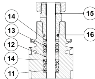
PTFE/GR V-Rings (V1.2)
