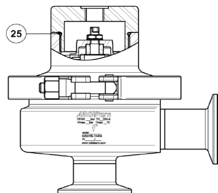
Dome-loaded top
