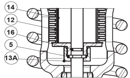
Detail B (DN 80 - DN 100)
