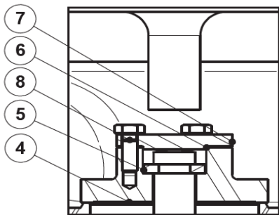
Detail A (DN 15 - DN 100)
