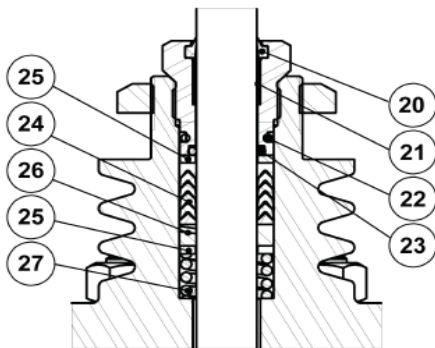
PTFE/GR V-RINGS (V1.2)
