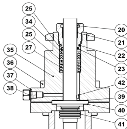
BELLOWS SEALING (BV1)
