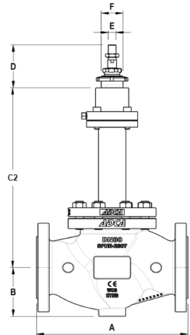
Bellows sealed valve
