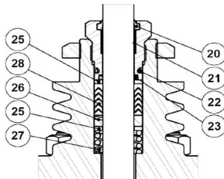
PTFE V-RINGS (V2.2)
