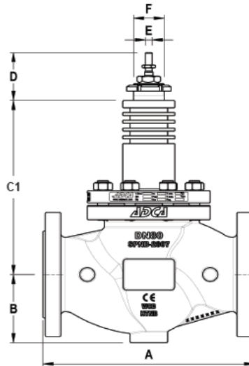
Valve with extended bonnet
