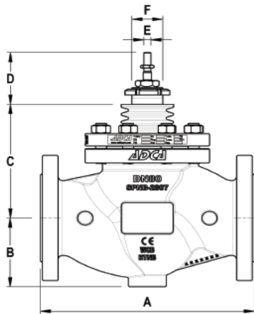
Valve with standard bonnet
