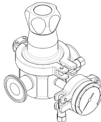
Optional pressure gauge connection.
