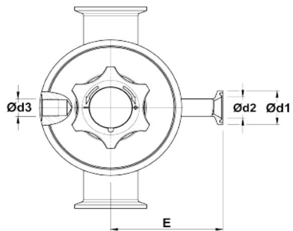
Optional pressure gauge connection.
