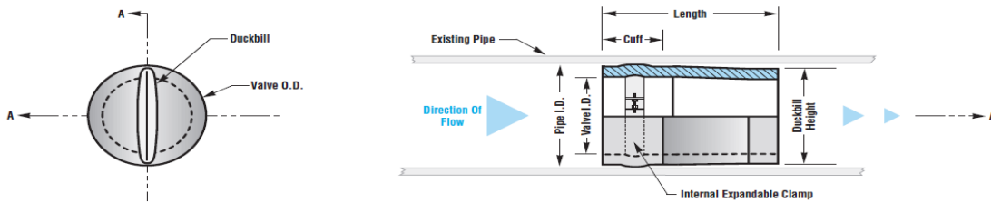
Detail of ProFlex In-Line Slip-In Rubber Check Valve; Style 740
