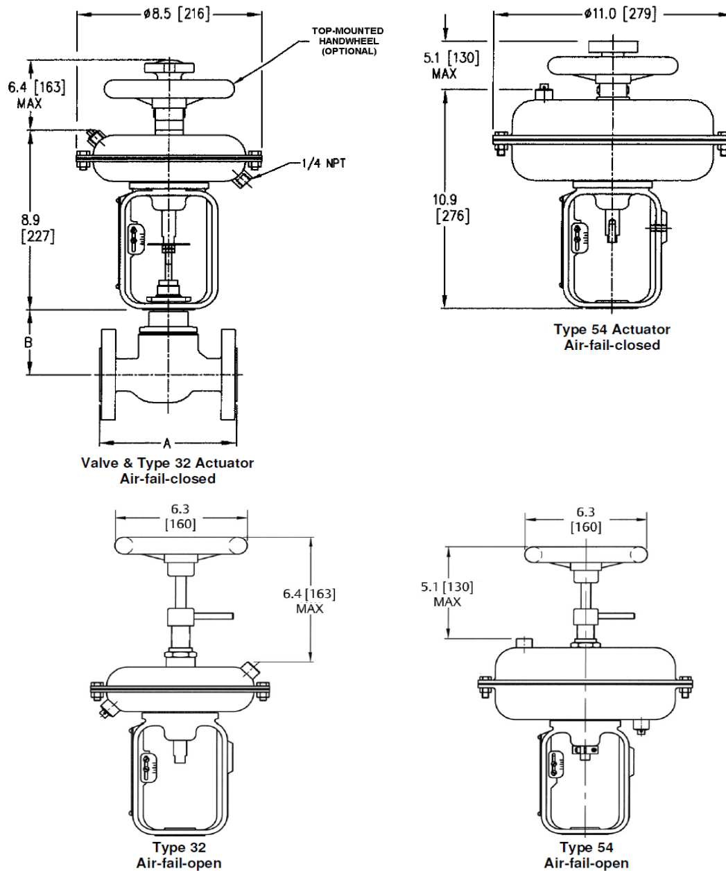
Figure 3. DIMENSIONS: ins [mm]
