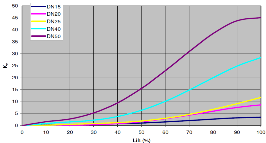
Figure 2. - K v vs. Valve Lift
