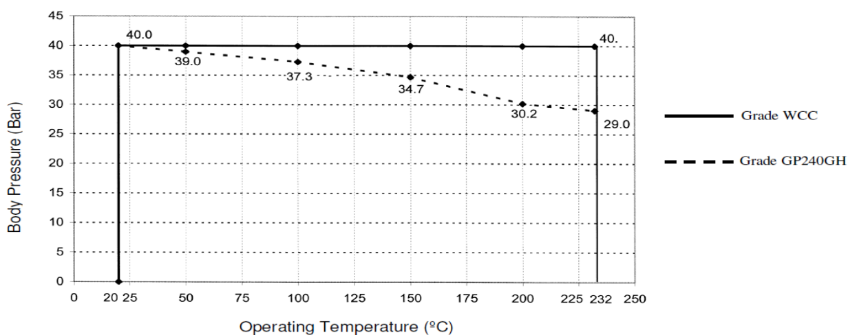
Figure 1. Body Pressure - Temperature Rating
